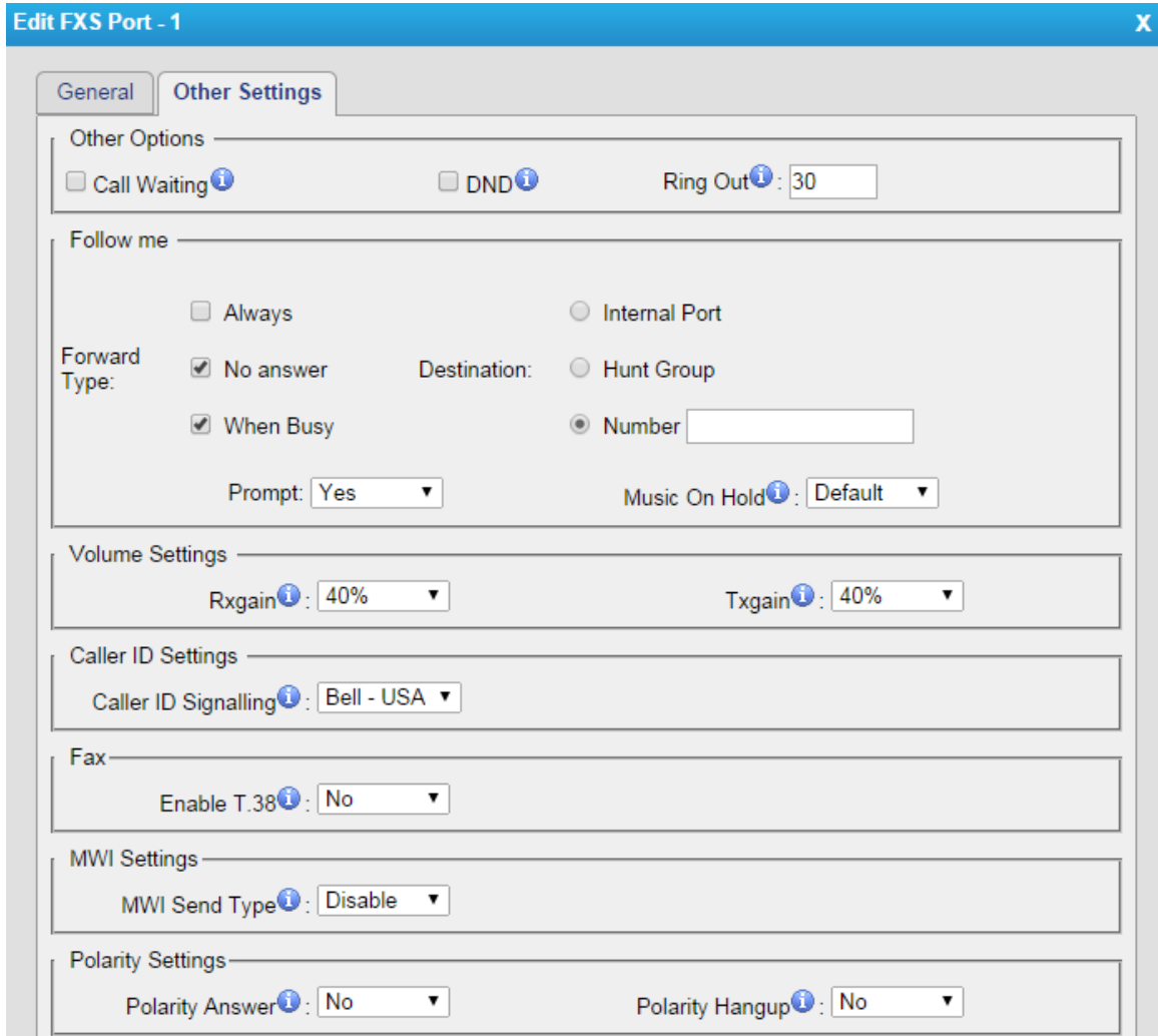
Figure 4-3 FXS Port Other Settings
