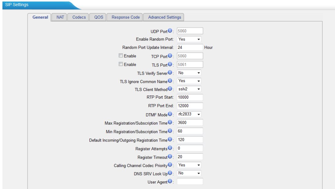
Figure 4-12 SIP General Settings
